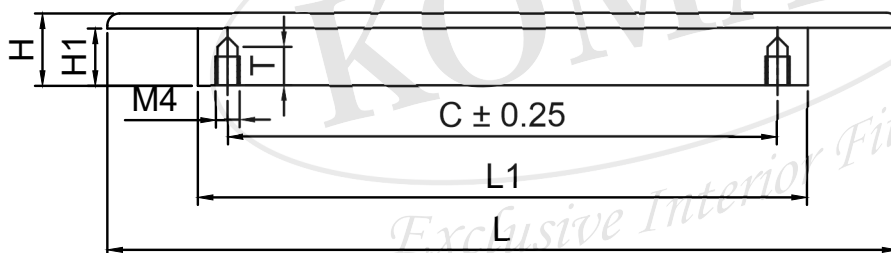
FRONT View
