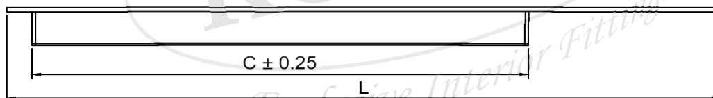
FRONT View
