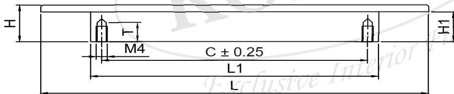
FRONT View
