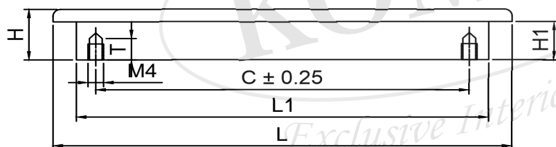
FRONT View
