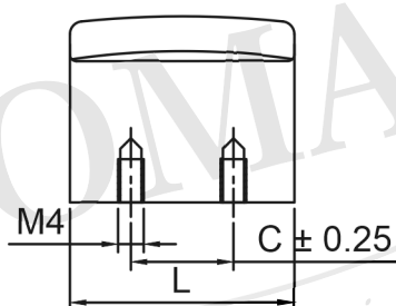
BACK VIEW
